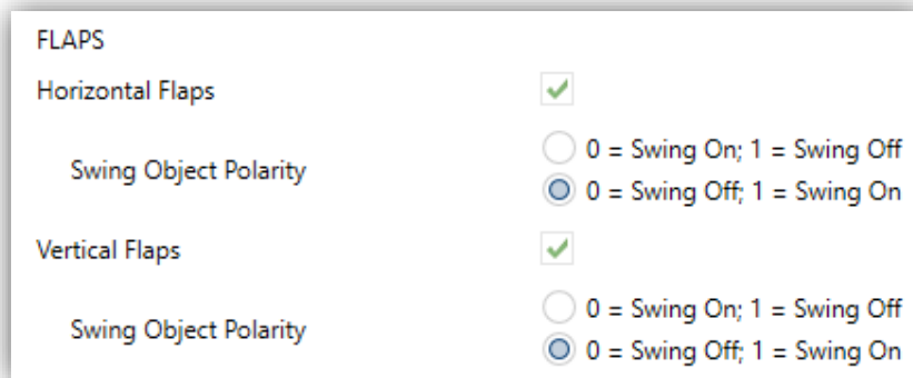
Figure 6. AC Gateway. Configuration. Flaps.
