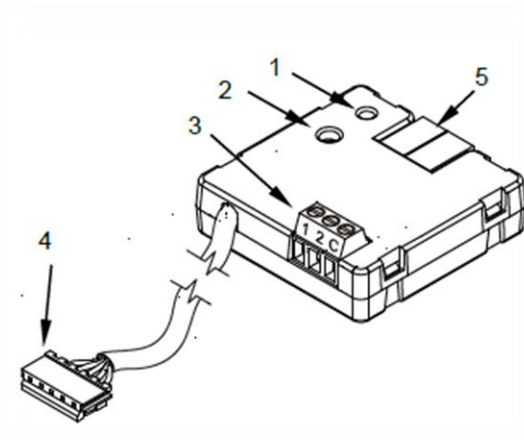
Figure 1. Element scheme.
